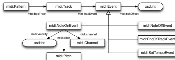
Fig. 1. Data model of MIDI concepts and their relations: patterns, tracks, events, and their attributes.
